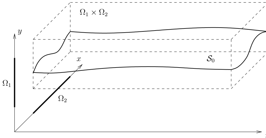
FIGURE 2. \mathcal{S}_0 is bounded away from \partial\Omega_2 uniformly in t \in \mathbb{R} .
