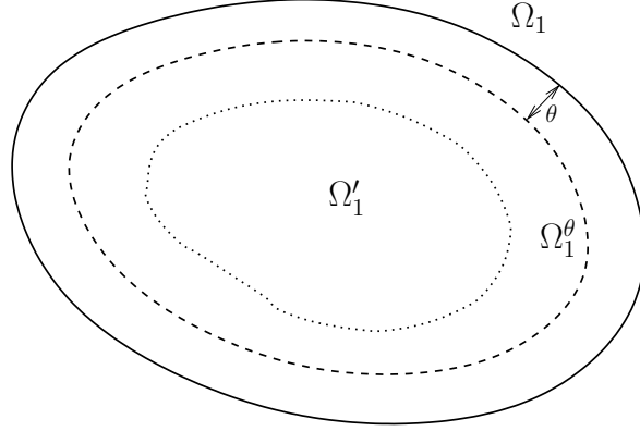
FIGURE 3. For \theta > 0 small enough the boundary of \Omega_1^\theta is C^m and \Omega_1' \subset \Omega_1^\theta \subset \Omega_1 .
