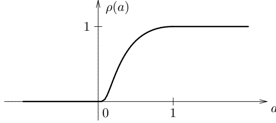
FIGURE 1. C^\infty cut-off function \rho : \mathbb{R} \rightarrow [0, 1]
